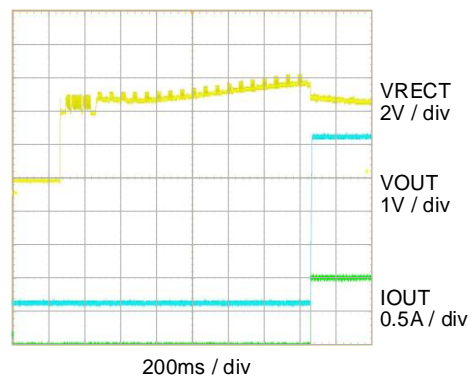
BPP, V_{OUT} = 5V , Startup With 1A Load
