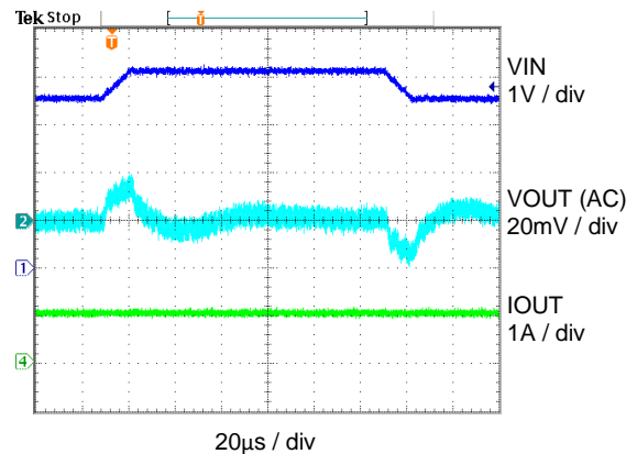
Line Transient Response ( V_{OUT} = 1.15625V , Mode = FPWM)
